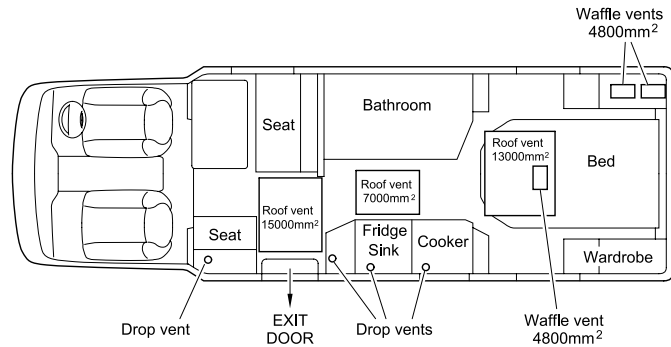
Ventilation - Roadstar TI
