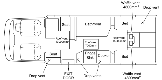
Ventilation - Roadstar EB
