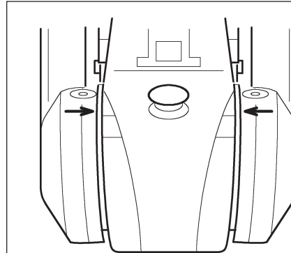
Fig 6 Friction pads worn out and need replacing
